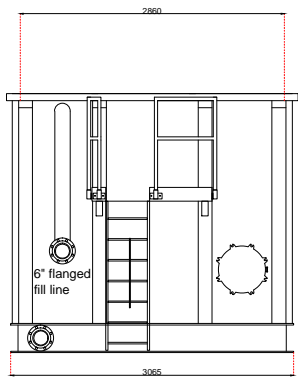
6" flanged outlet 450mm quick release manway
